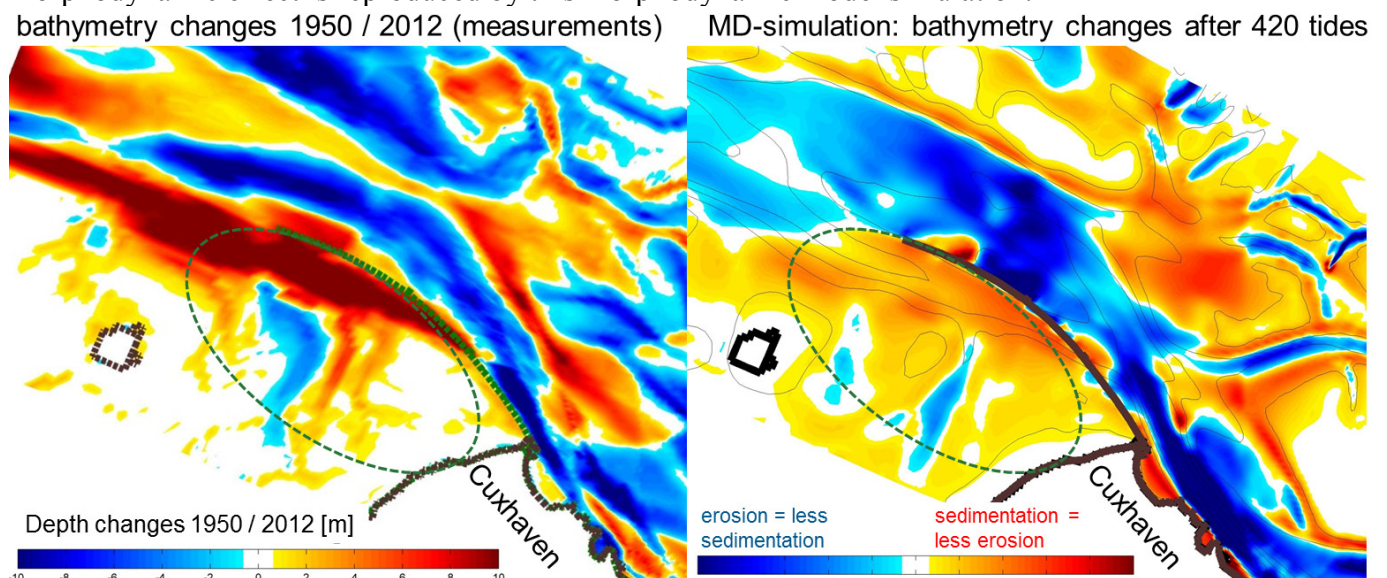
Figure 4. Bathymetry changes 1950/2012 in comparison to a morphodynamic run over 420 tides
